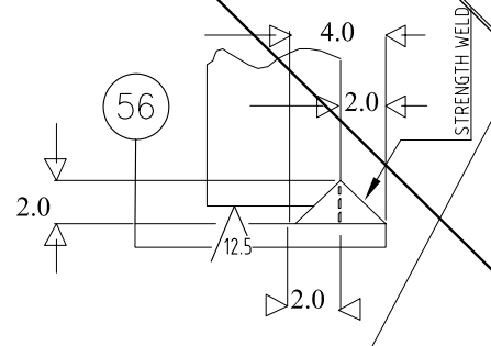
TUBESHEET/TUBE DETAIL
